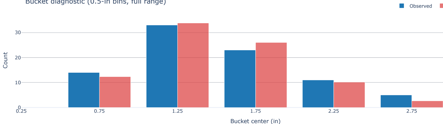
Bucket diagnostic (0.5-in bins, full range)
