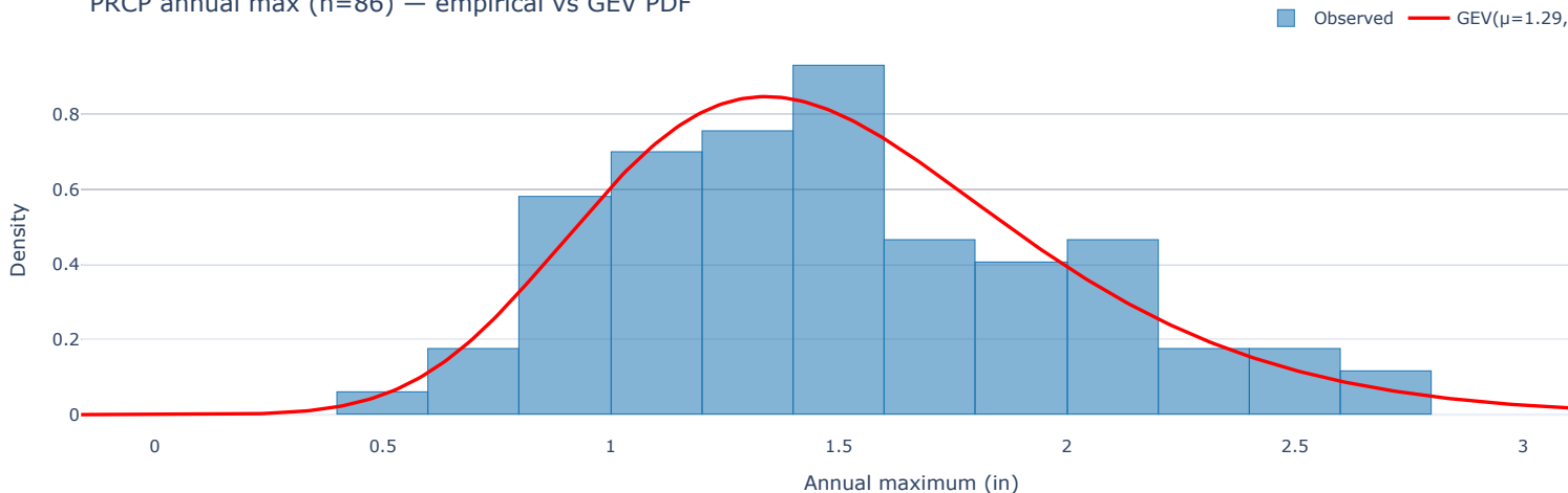
PRCP annual max (n=86) — empirical vs GEV PDF
