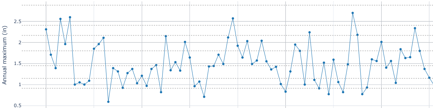
PRCP annual max (n=86) with fitted percentiles
